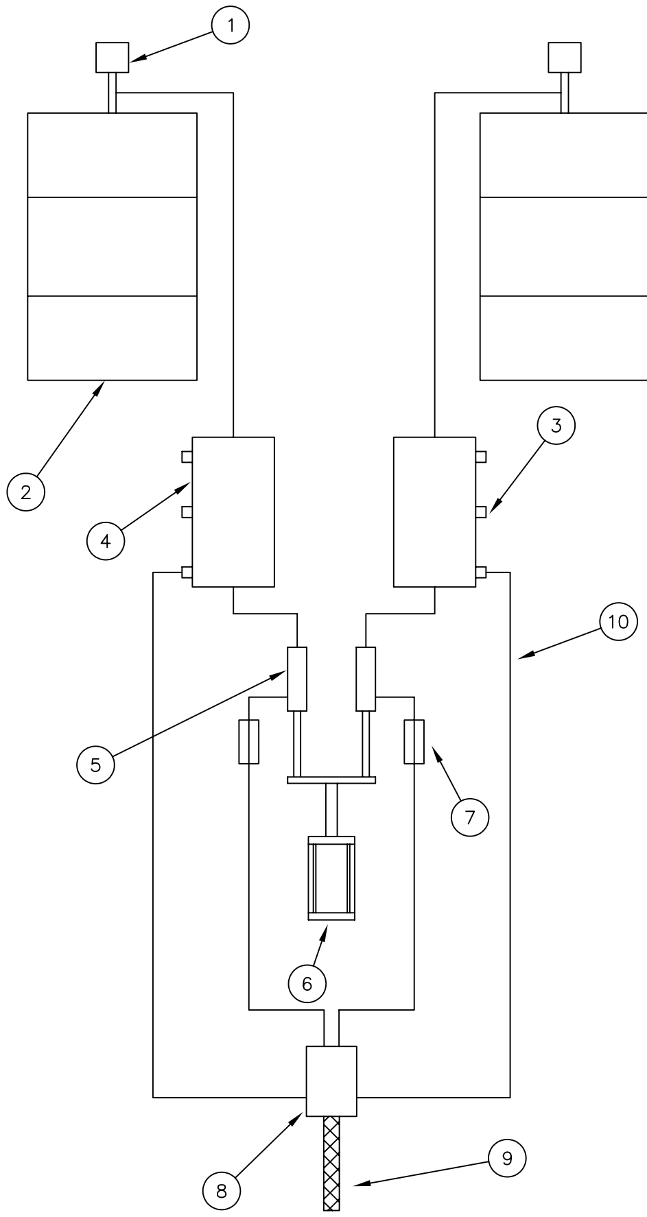
SYSTEM LAYOUT, CMP METER
